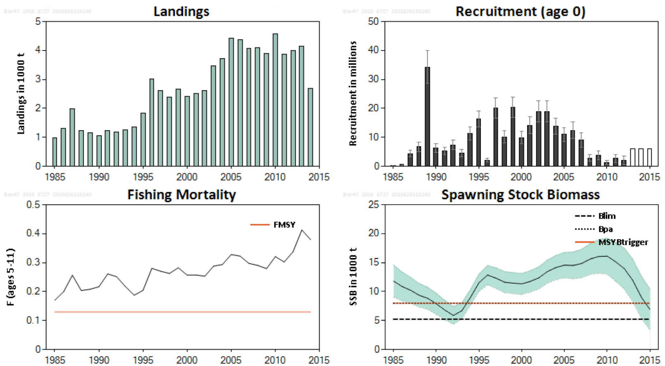
Figure 1: Seabass in the southern North Sea, Irish Sea, English Channel, and Celtic Sea. Summary of stock assessment (weights in thousand tonnes). Landings are from the commercial fishery only. Fishing mortality is shown for the combined commercial and recreational fisheries (ICES 2015a).
