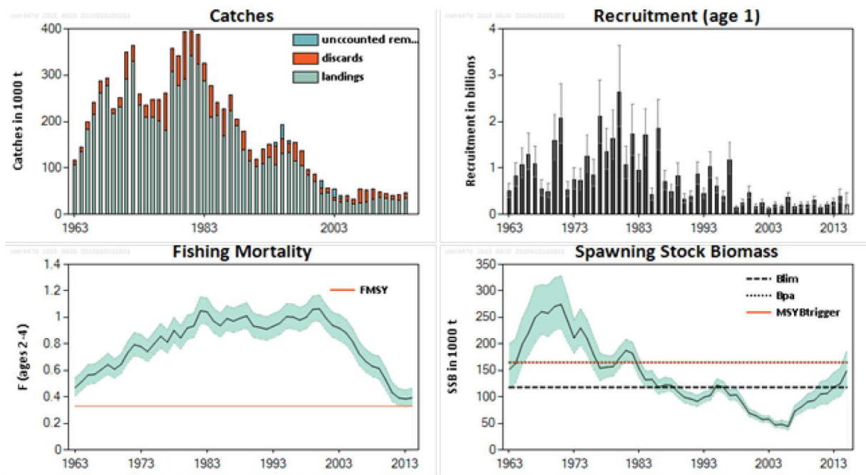
Figure 2. Cod in the North Sea, eastern English Channel and Skagerrak. Summary of stock assessment with point-wise 95% confidence intervals (ICES, 2015b). Any observed changes over the past decade, including any extremes.
